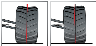
Positive Camber
